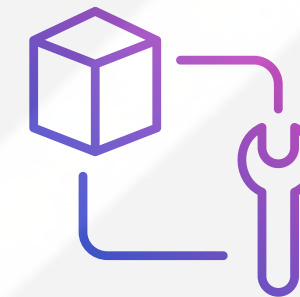
Blockchain Maintenance
